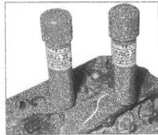
FREEZE-CRACKS
