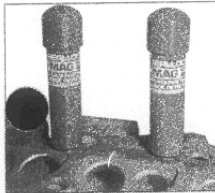
VALVE-PORT CRACKS
